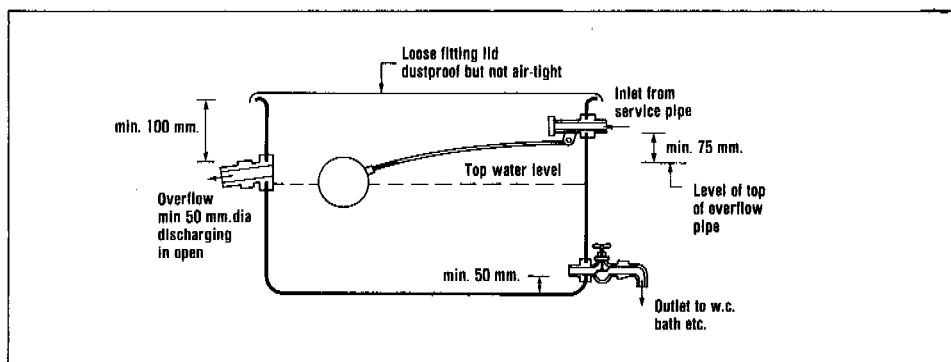
Figure 3. Domestic water storage tank.
