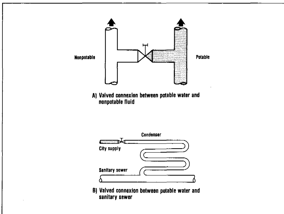
Figure 8. Elements of a cross-connexion.
