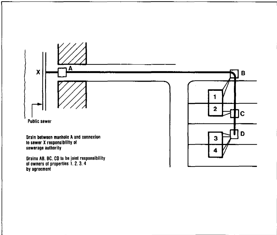
Figure 1. Situation requiring combined drainage agreement.
