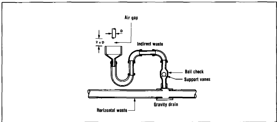
Figure 14. Indirect waste arrangement.
