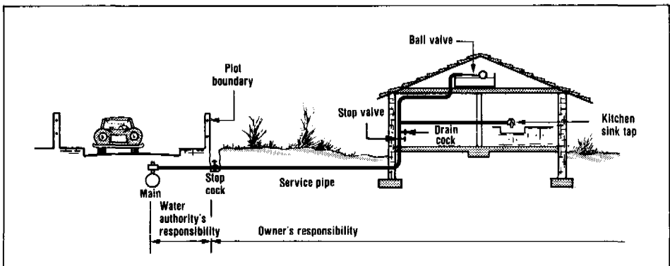
Figure 5. Water service to a domestic system.
