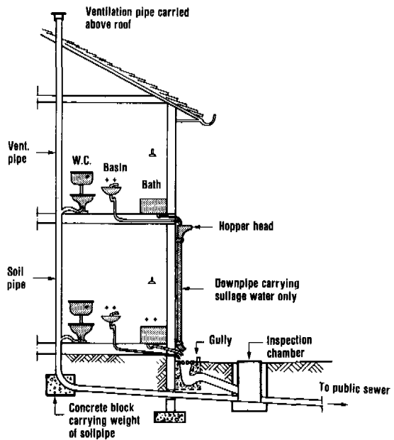
B. Principle of the 'two-pipe' system.
