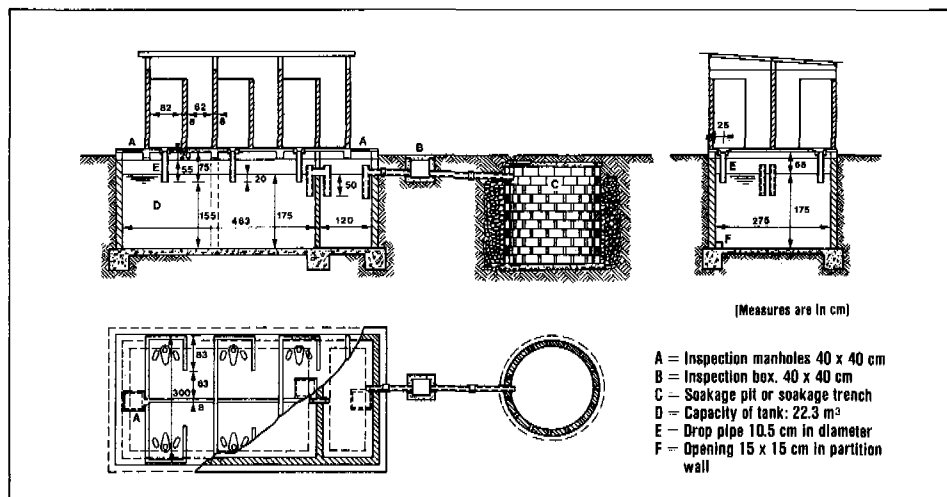
Figure 16. Communal aqua-privy.
