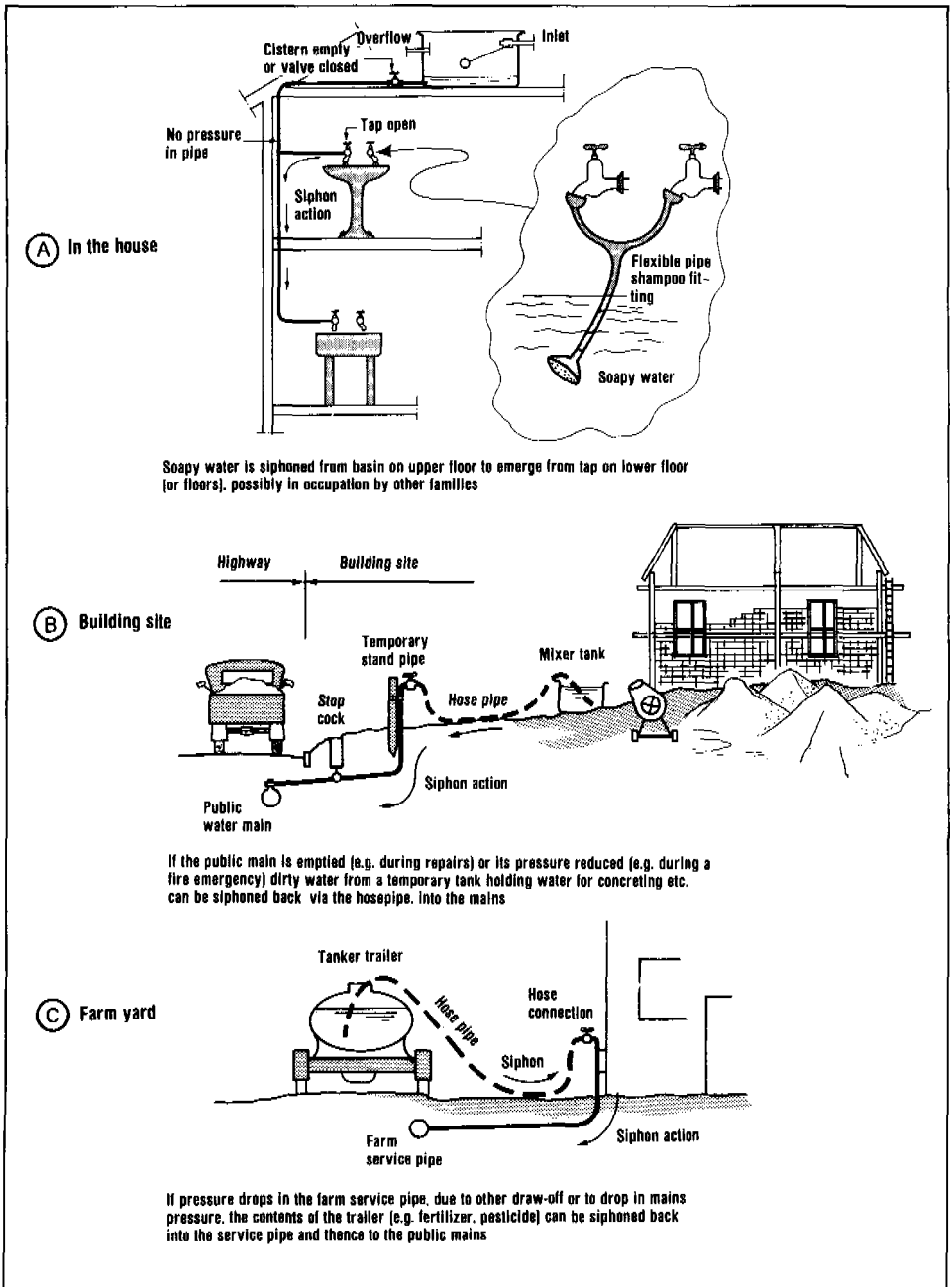
Figure 9. Ways in which back siphonage can occur.
