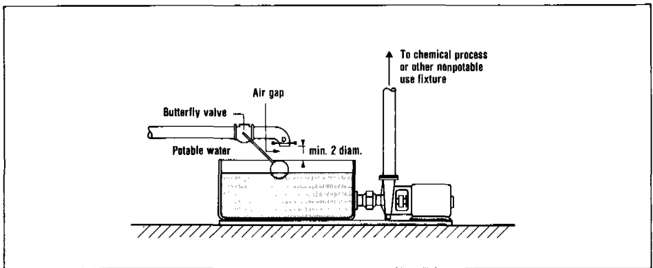
Figure 7. Air gap protection against cross-connexion.
