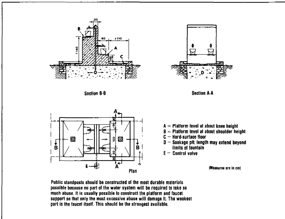
Figure 17. Possible arrangement of public standpost.
