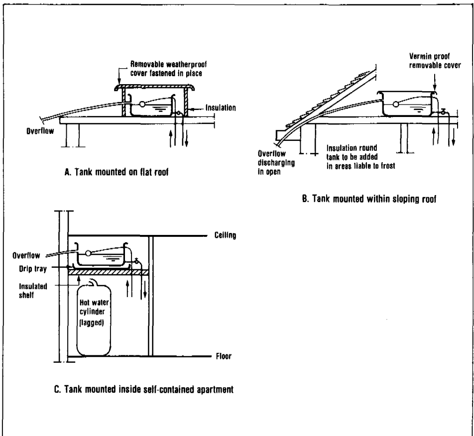
Figure 4. Water storage tanks.
