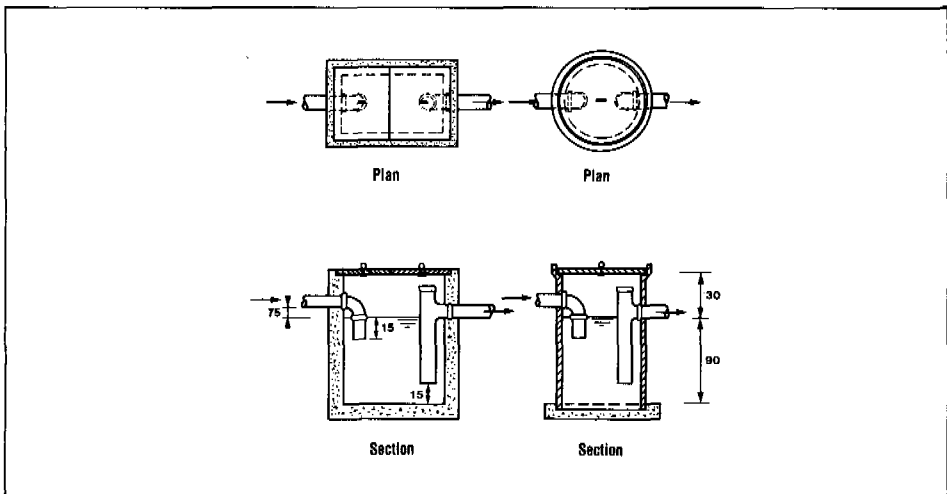
Figure 12. Typical grease traps.
