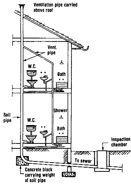
A. Principle of the 'one-pipe' system.
