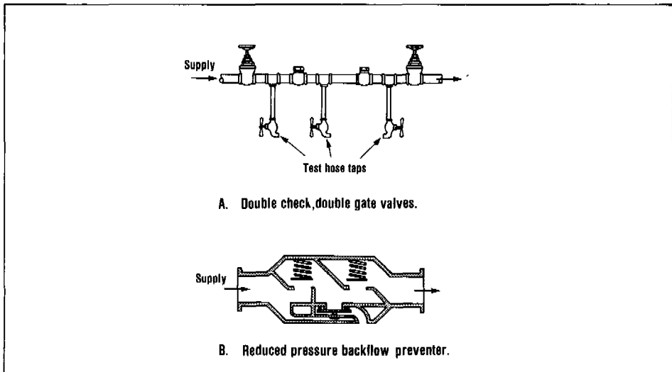
Figure 10. Backflow prevention devices.
