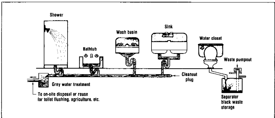
Figure 15. Greywater-blackwater system.
