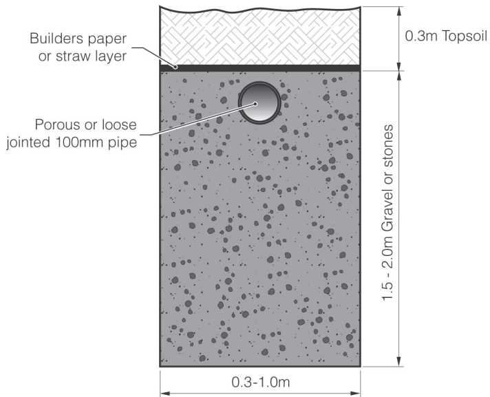
Figure 7.17. Soakfield trench
