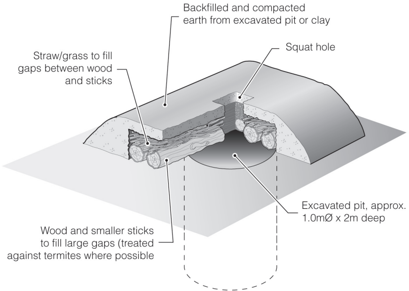
Figure 7.1. Traditional latrine using local materials
