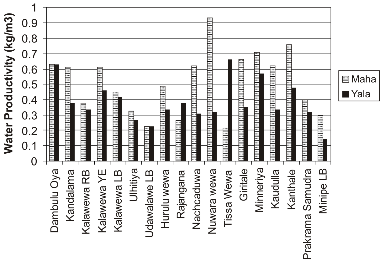
Figure 28. Water productivity in selected irrigation schemes
