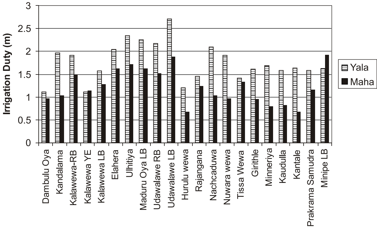
Figure 27. Irrigation duty in selected major irrigation schemes
