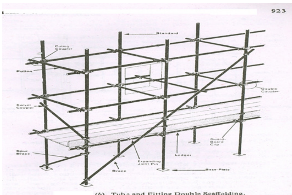
Fig.16 Steel scaffolding.
