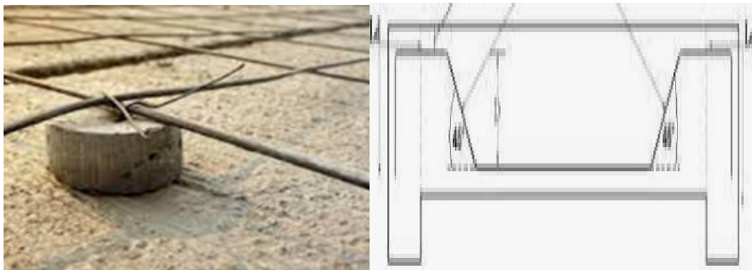
Fig.24: Concrete spacer and bar chain
