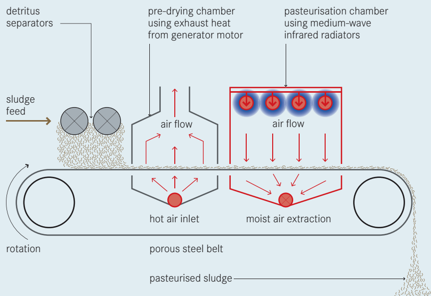
Figure 6: Schematic of the LaDePa sludge pelletizer
