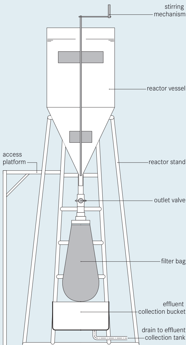
Figure 7: Schematic of a struvite reactor with stirring mechanism and filter bag
