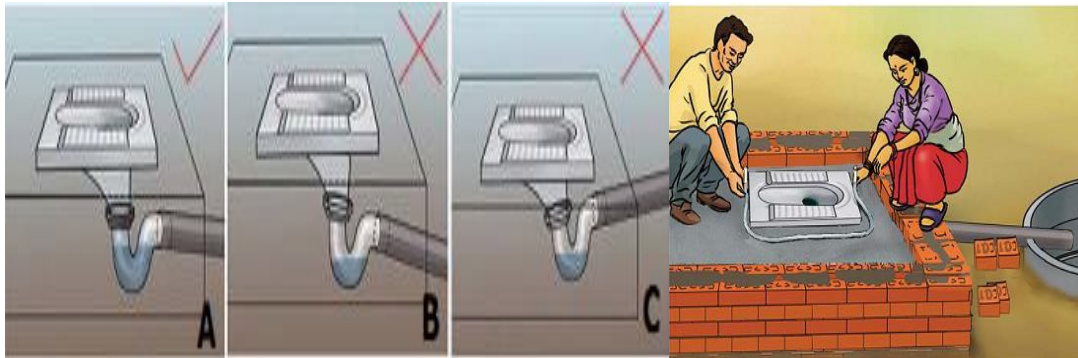
Figure-4.5: The position of the pan and siphon, check by water level
