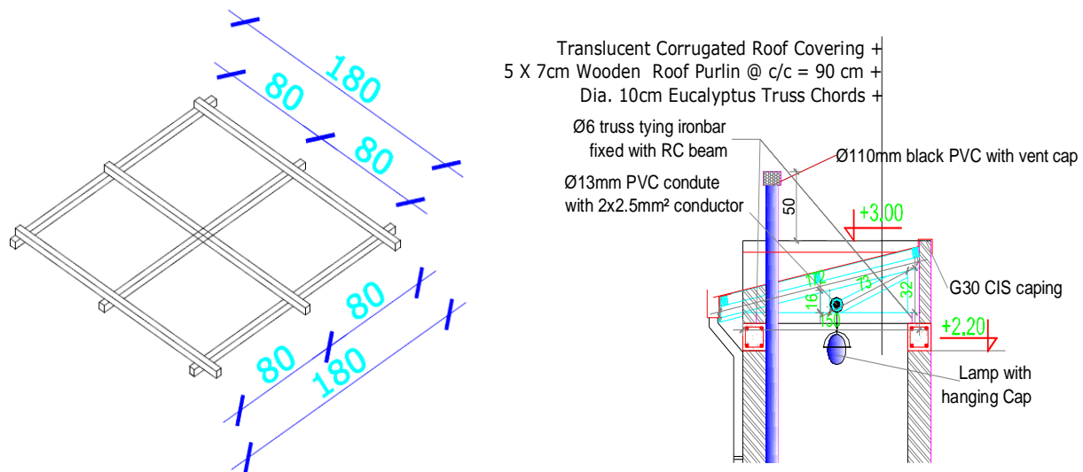
Fig. 5.1. Roof Structure
