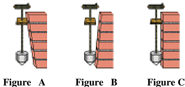
Figure.3.15 checking vertical alignment with plumb bob
