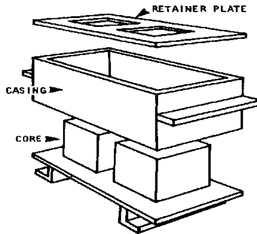
Figure-1.4. Mold made out of lumber
