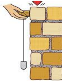
Figure.3.4 Checking Vertical Alignment of Wall
