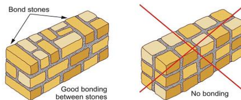
Figure.3.3. Vertical Alignments of Bonding between stones
