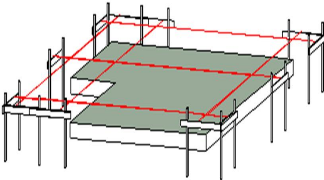
Figure-1: Setting out
