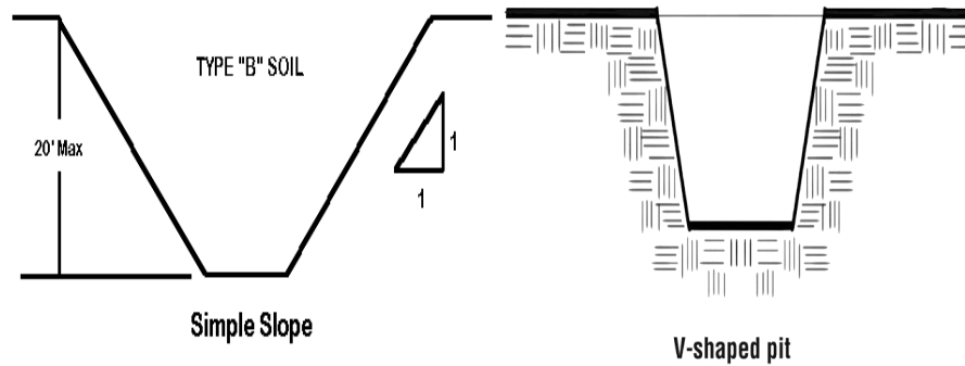
Figure-6: Excavation collapse prevention slope method
